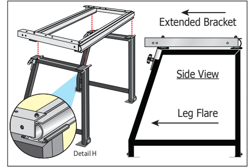
Rail Assembly
