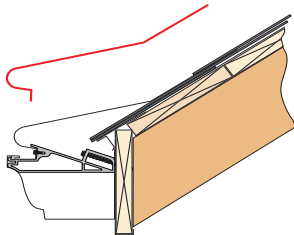
8/12 Pitch-Over Shingle
