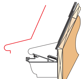
18/12 Pitch-Mansard
