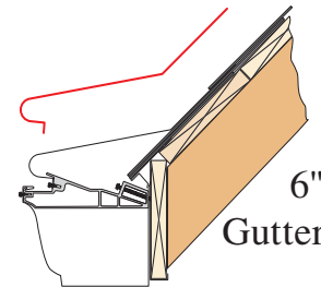
12/12 Pitch-Over Shingle
