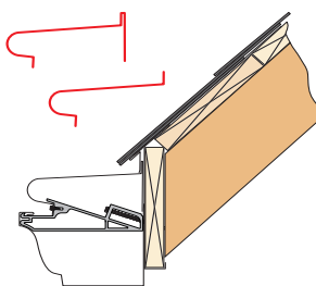
12/12 Pitch-Fascia Mount
